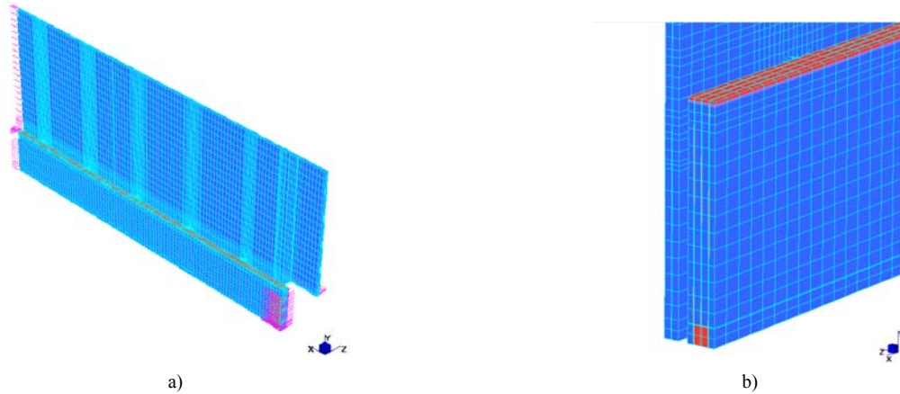
Fig. 7a) Isometric view and b) detail of the mid cross-section of the beam and railings in the second FE model.
